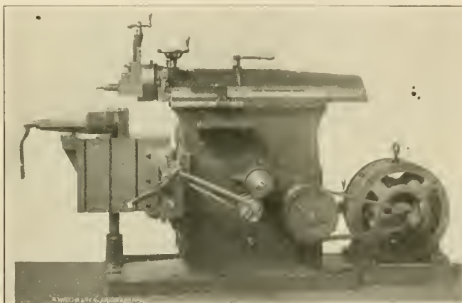
CINCINNATI SHAPER COMPANY'S CRANK SHAPER.
